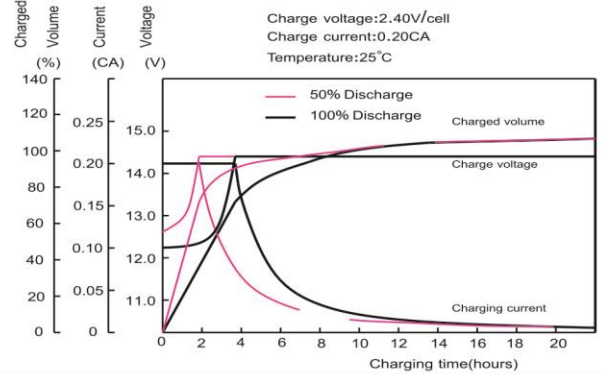
Charging characteristic (25°C)
