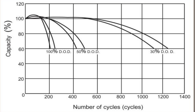
Cycle Life on D.O.D (25°C)
