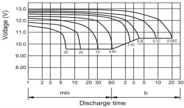
Discharge characteristic (25°C)
