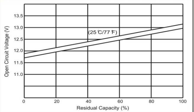
The relationship for OCV and Capacity (25°C)
