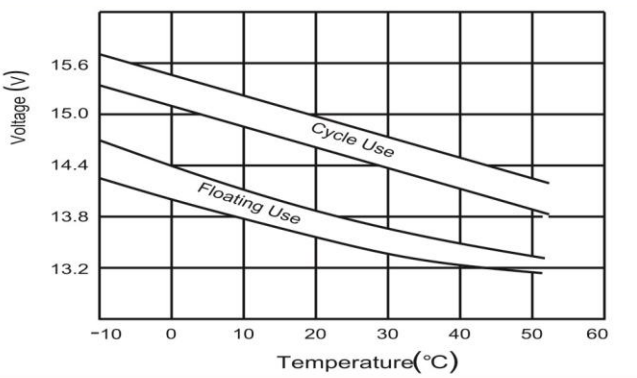
The relationship for Charging voltage and Temperature
