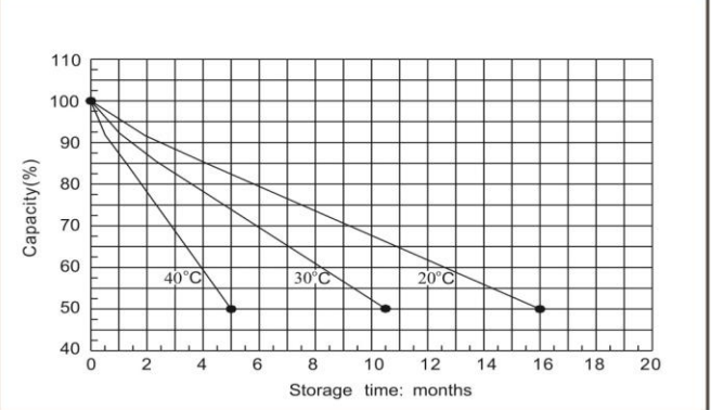
Self-discharge characteristic
