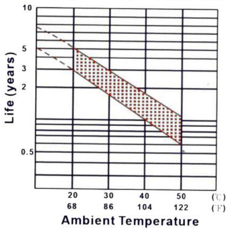
Trickle (or float) Service Life
