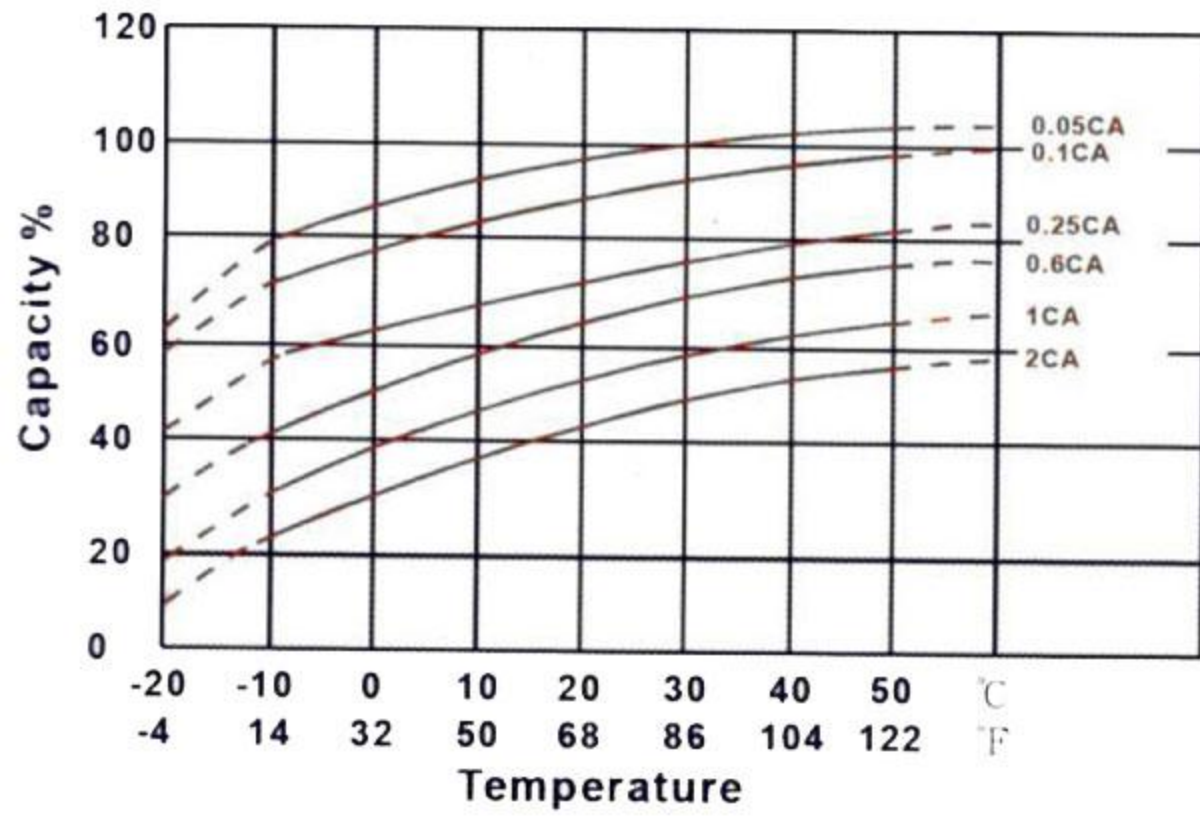
Effect of Temperature on Capacity 25°C (77°F)
