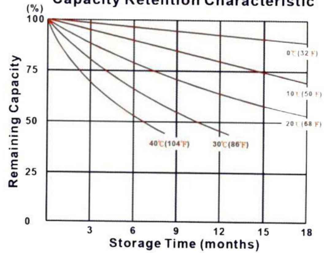
Capacity Retention Characteristic
