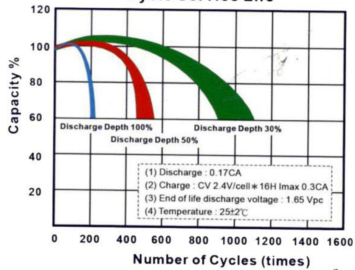
Cycle Service Life
