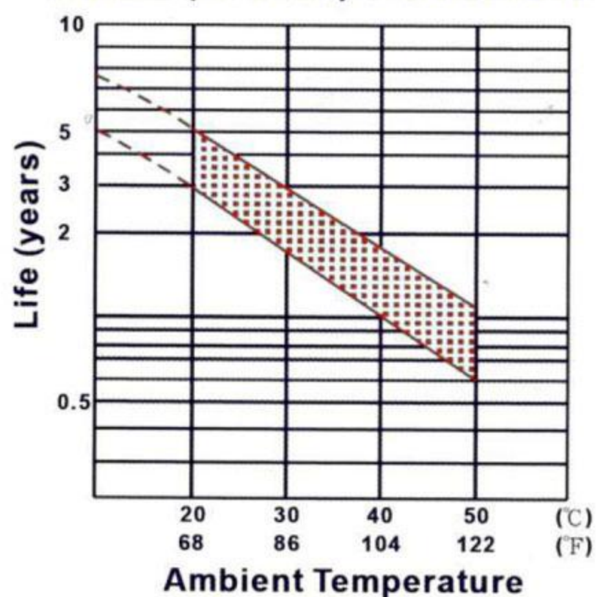
Trickle (or float) Service Life
