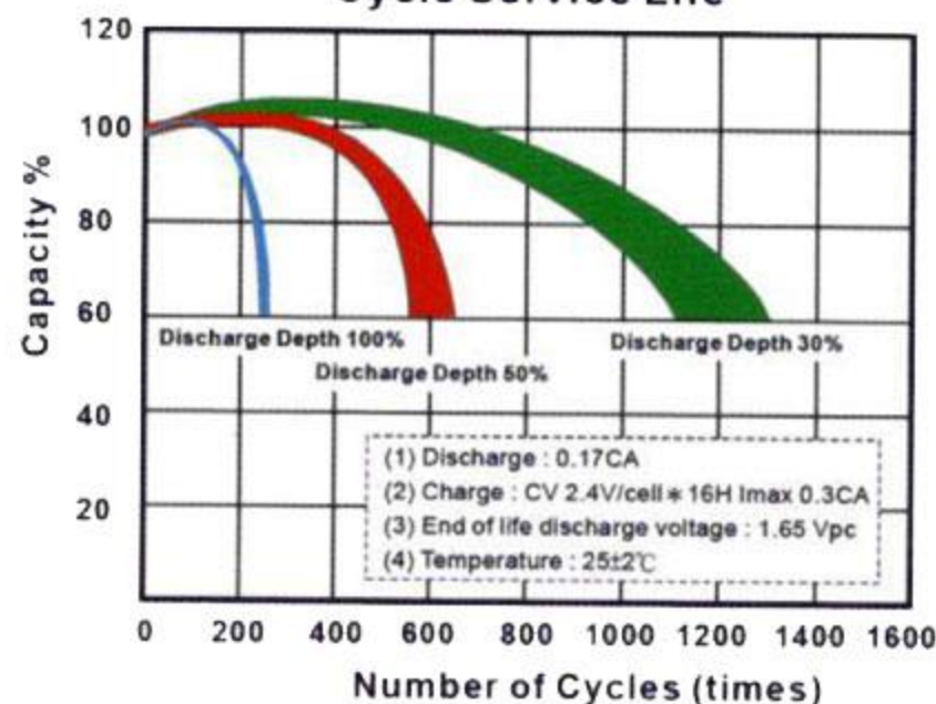
Cycle Service Life
